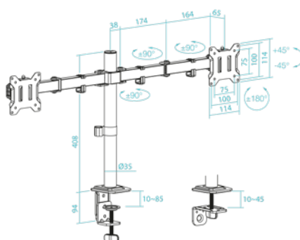
Dimensions (mm)
