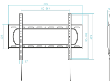
Dimensions (mm)
